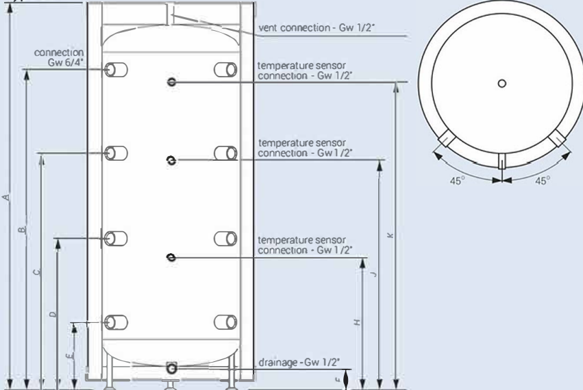
type SVW with coil
