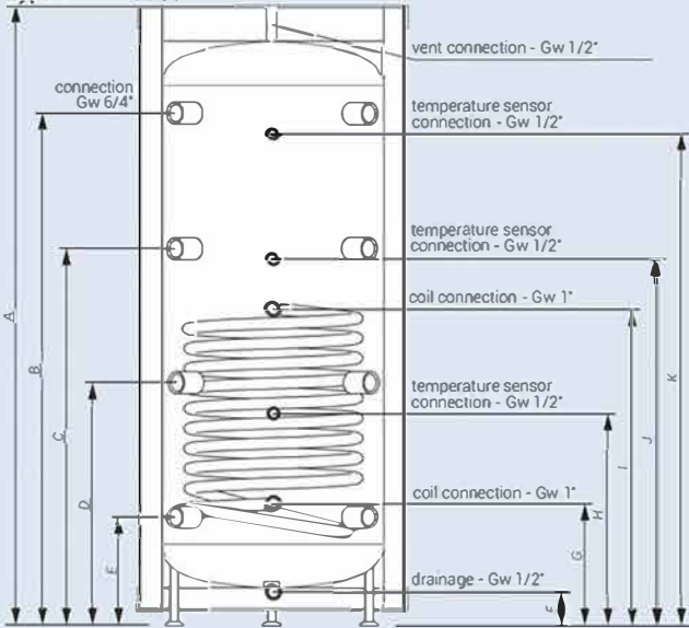
type SVW with coil
